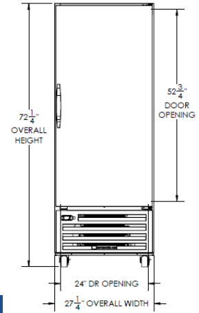
Elevation View
